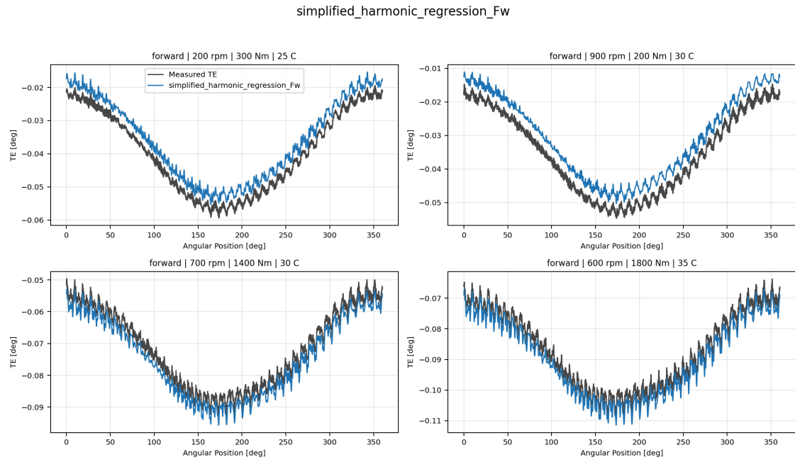
simplified_harmonic_regression_Fw measured-versus-predicted TE collage
