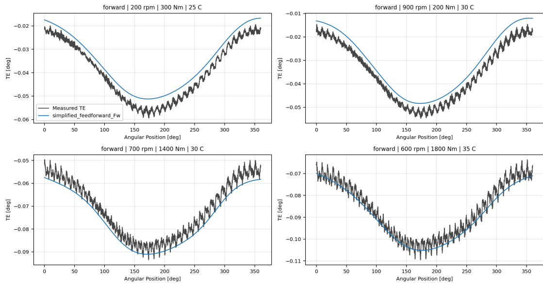
simplified_feedforward_Fw measured-versus-predicted TE collage
