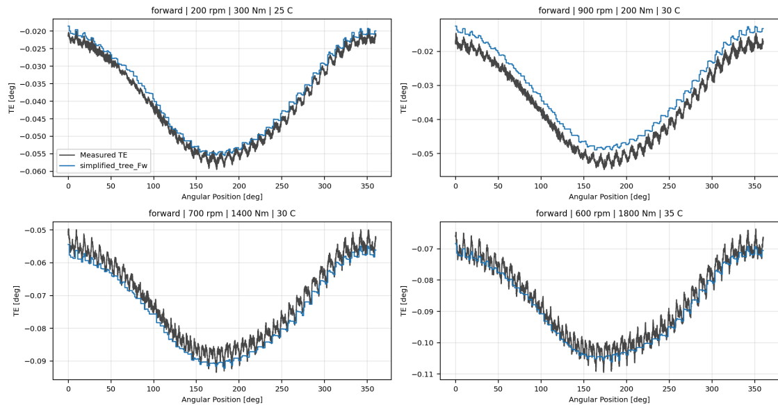
simplified_tree_Fw measured-versus-predicted TE collage
