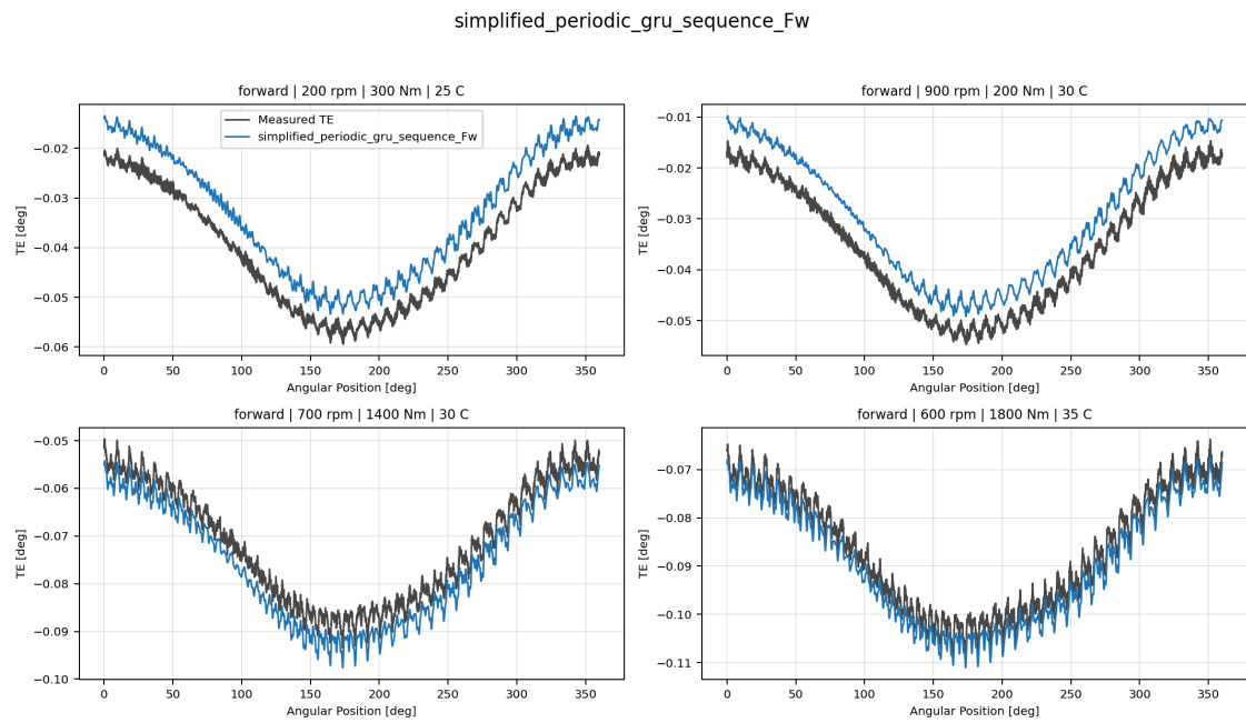
simplified_periodic_gru_sequence_Fw measured-versus-predicted TE collage
